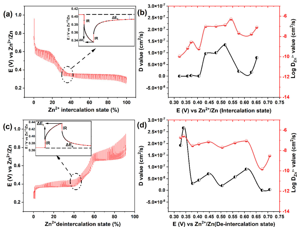
Fig. 5 Galvanostatic intermittent titration technique (GITT) curves of in 2 M ZnSO_4 at 0.1 A g^{-1} recorded during the Zn^{2+} intercalation (a) and deintercalation process (c) as a function of state of (de)intercalation process. The insets in (a) and (c) scheme for a single step of a GITT experiment. The corresponding Zn^{2+} diffusion coefficients values among the selected steps during intercalation (b) and deintercalation (d) process.
