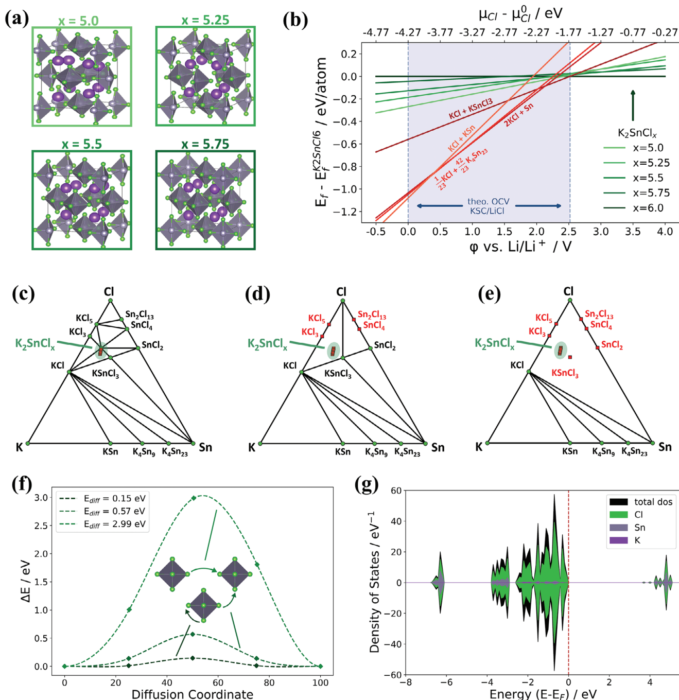
Figure 6. a) Crystal structure of reduced KSC. b) Grand canonical phase diagram of K_2SnCl_x and its decomposition products. c–e) K–Sn–Cl ternary phase diagrams at \phi = 4.27 V , \phi = 2.52 V , and \phi = 1 V versus Li/Li^+ where green/red datapoints represent E_{hull} = 0/E_{hull} > 0 . f) Diffusion barriers and g) density of states for pristine KSC.
