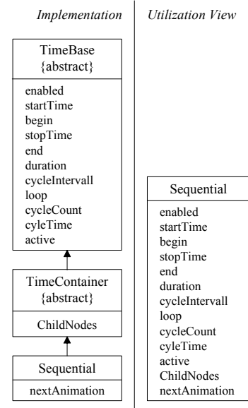
Figure 3. Inheritance in BEHAVIOR3D
