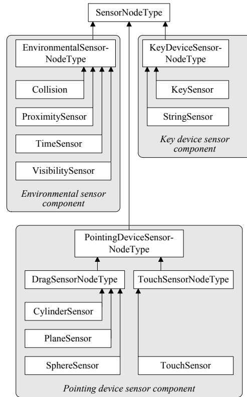
Figure 1. Part of the X3D SAI node hierarchy and grouping of nodes within X3D components
