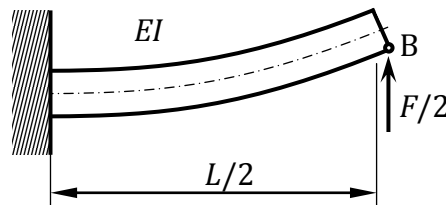
Fig. 1: Cantilever beam (half of beam under 3-point bending).
