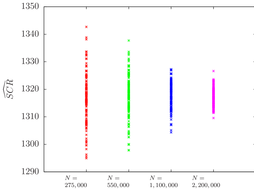
Figure 4: 120 simulations for different choices of N in the LSM Approach
