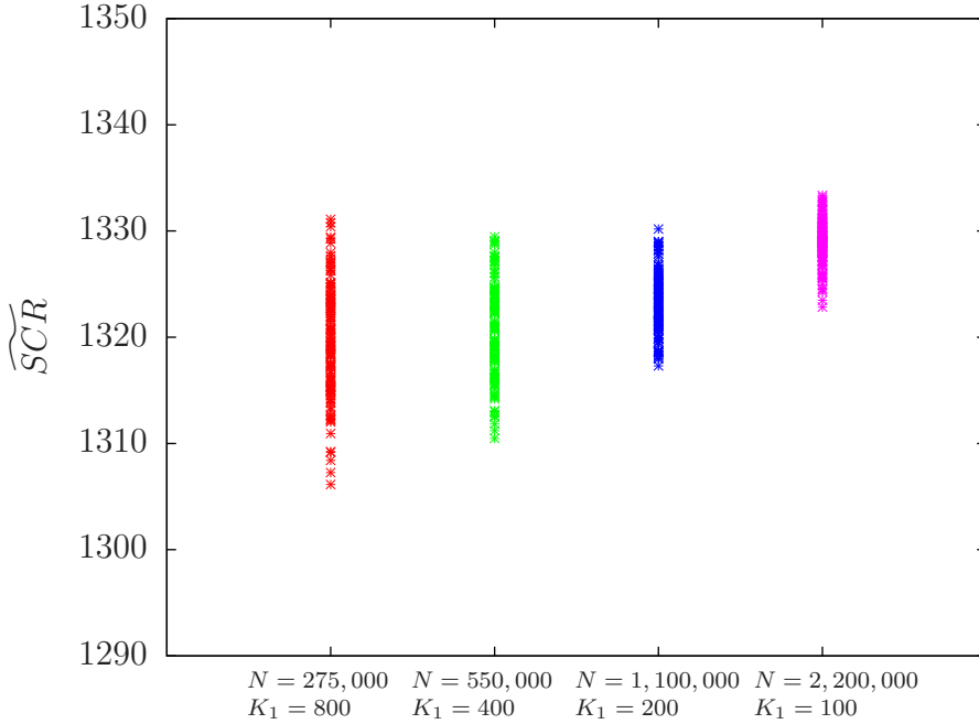
Figure 3: 120 simulations for different choices of N and K_1 , K_0 = 2,500,000 , Nested Simulations Approach
