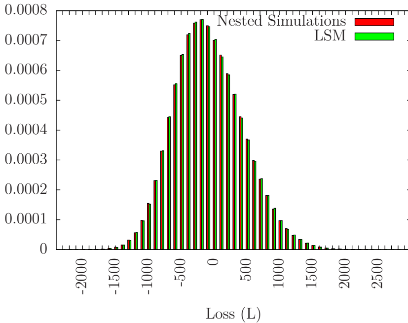
Figure 5: Empirical density functions for N = 550,000 and K_1 = 400
